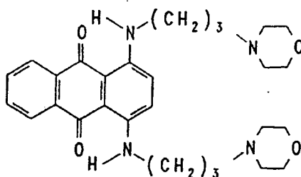
Compound 1c
